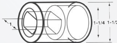
C1DD - 1" Double D x 1-1/4" smooth
