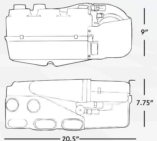
Dimension Detail
