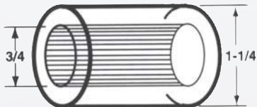
C736x2 - 3/4" 36 Spline only
