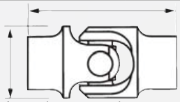
Single Joint 15/8" x 31/4" up to 35° angle
