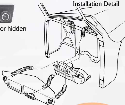
Installation Detail
