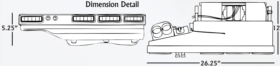
Dimension Detail
