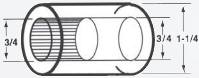
C736 - 3/4" 36 Spline x 3/4" smooth
